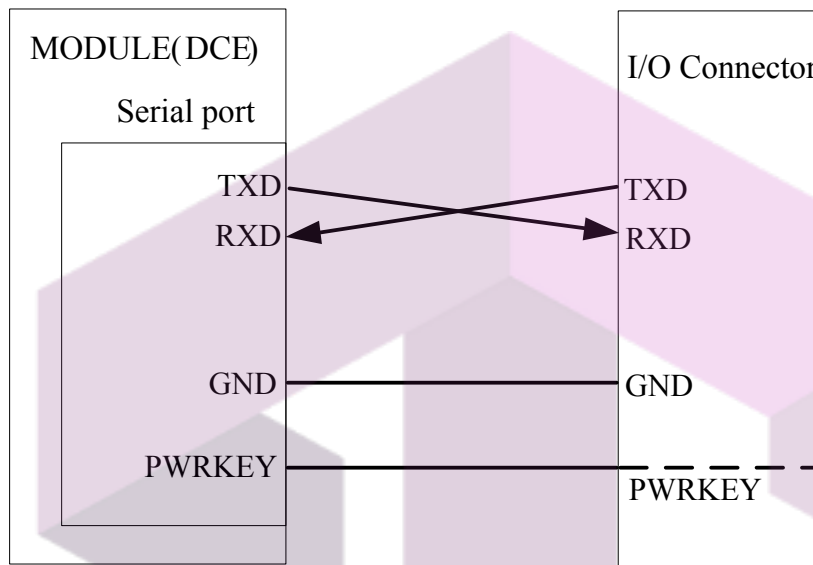
Figure 25: Connection for software upgrading and debugging
