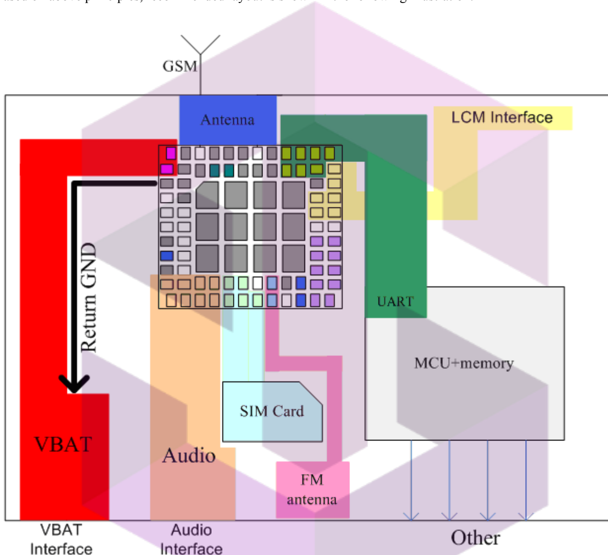
Figure 52: Recommended PCB layout
